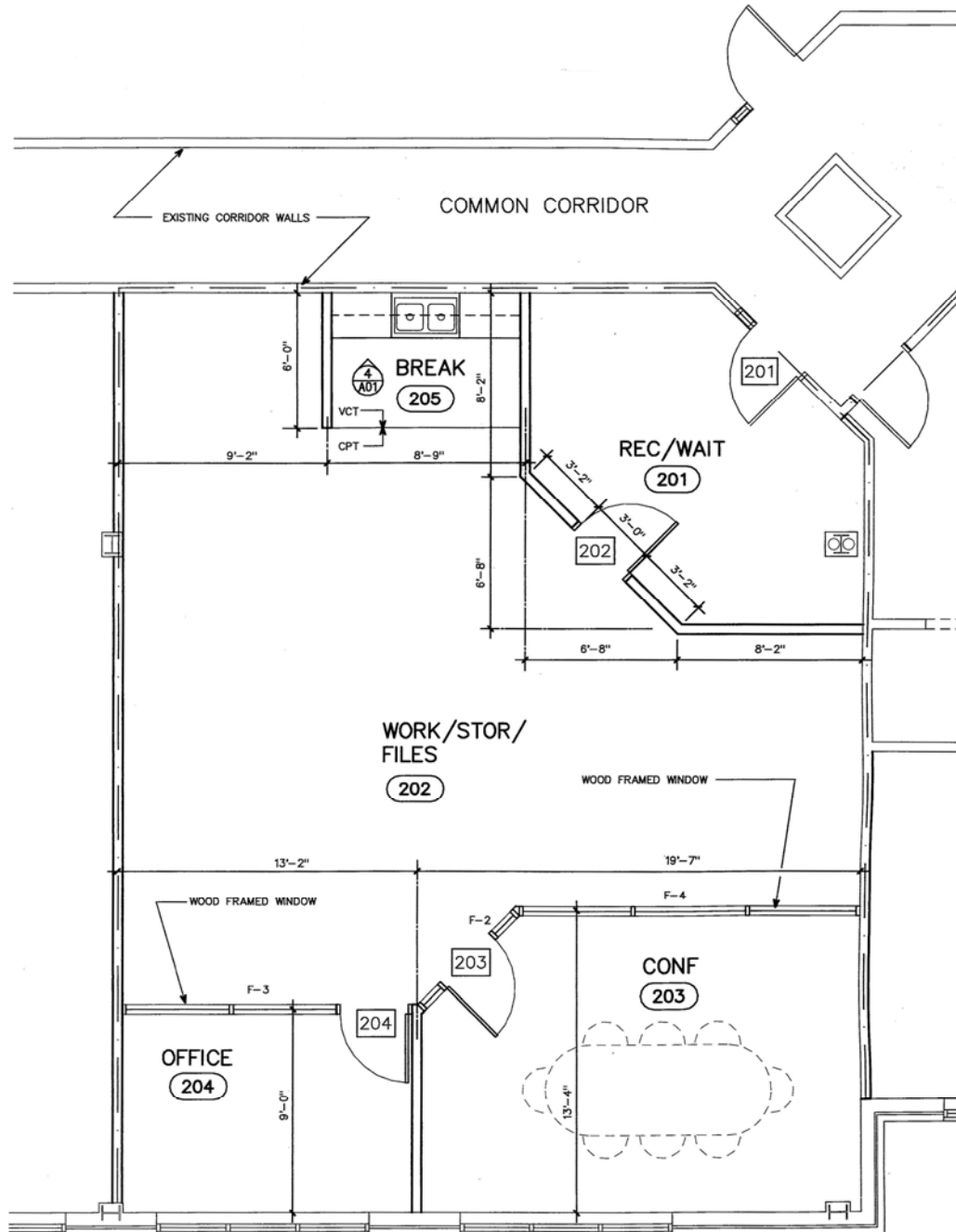
FLOOR PLAN - SUITE 220
